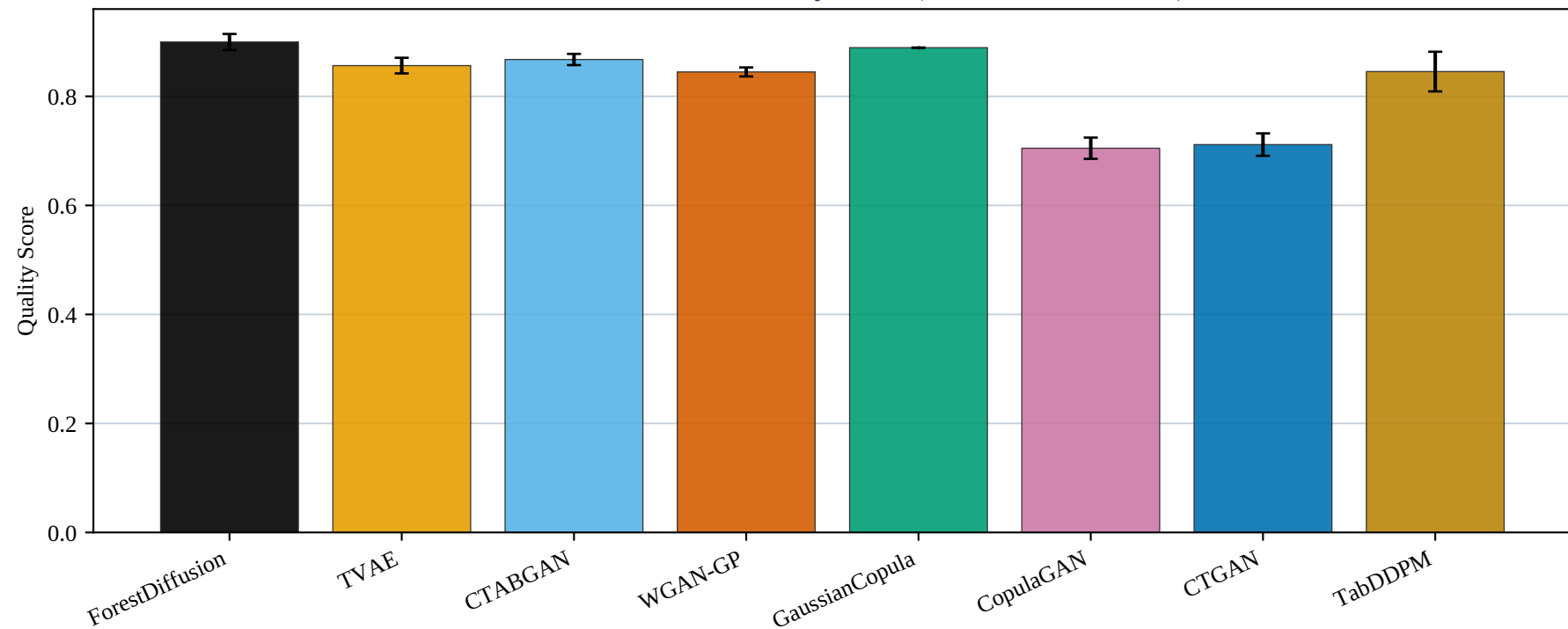
MAGIC Gamma — Quality Score (mean \pm SD, 10 seeds)
